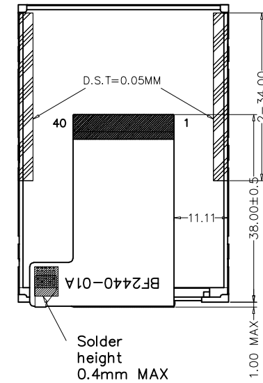
FPC Bending diagram FPC Launch shipment
