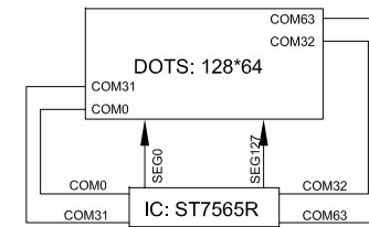
LCD LAYOUT
