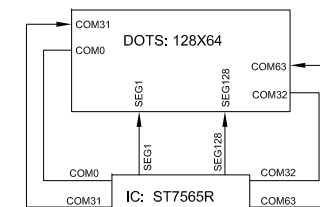
LCD LAYOUT
