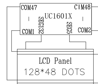
LCD Circuit Diagram
