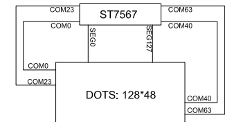
LCD LAYOUT
