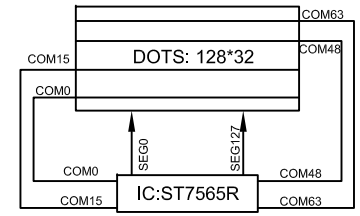
LCD LAYOUT
