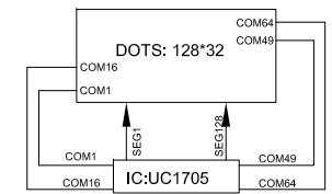
LCD LAYOUT
