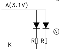
BACKLIGHT CIRCUIT 2PCS WHITE LEDS
