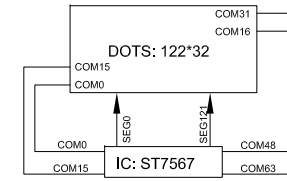
LCD LAYOUT
