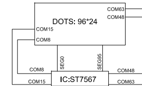
LCD LAYOUT
