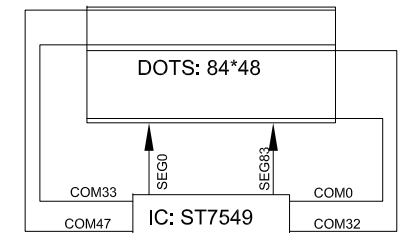
LCD LAYOUT
