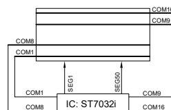
LCD LAYOUT
