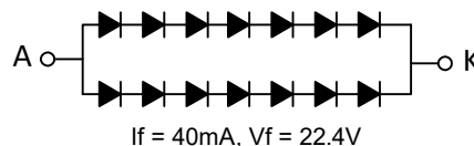
Backlight Circuit Diagram
