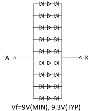
BACKLIGHT CIRCUIT DIAGRAM
