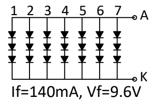
Backlight Circuit Diagram
