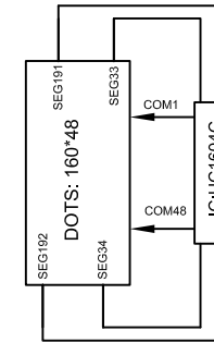
LCD LAYOUT
