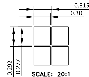
LCD LAYOUT
