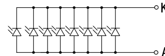
Backlight circuit
